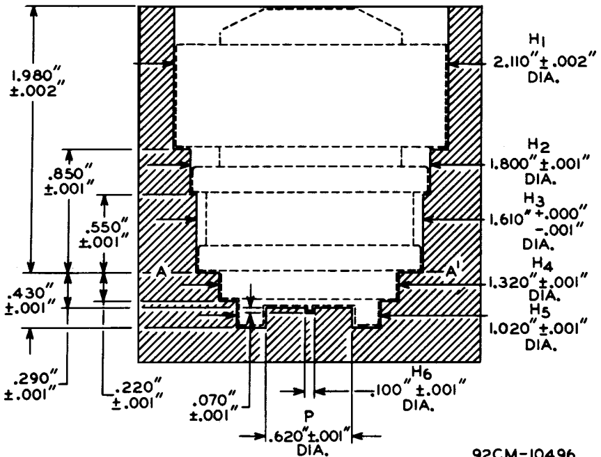
SKETCH G 1
